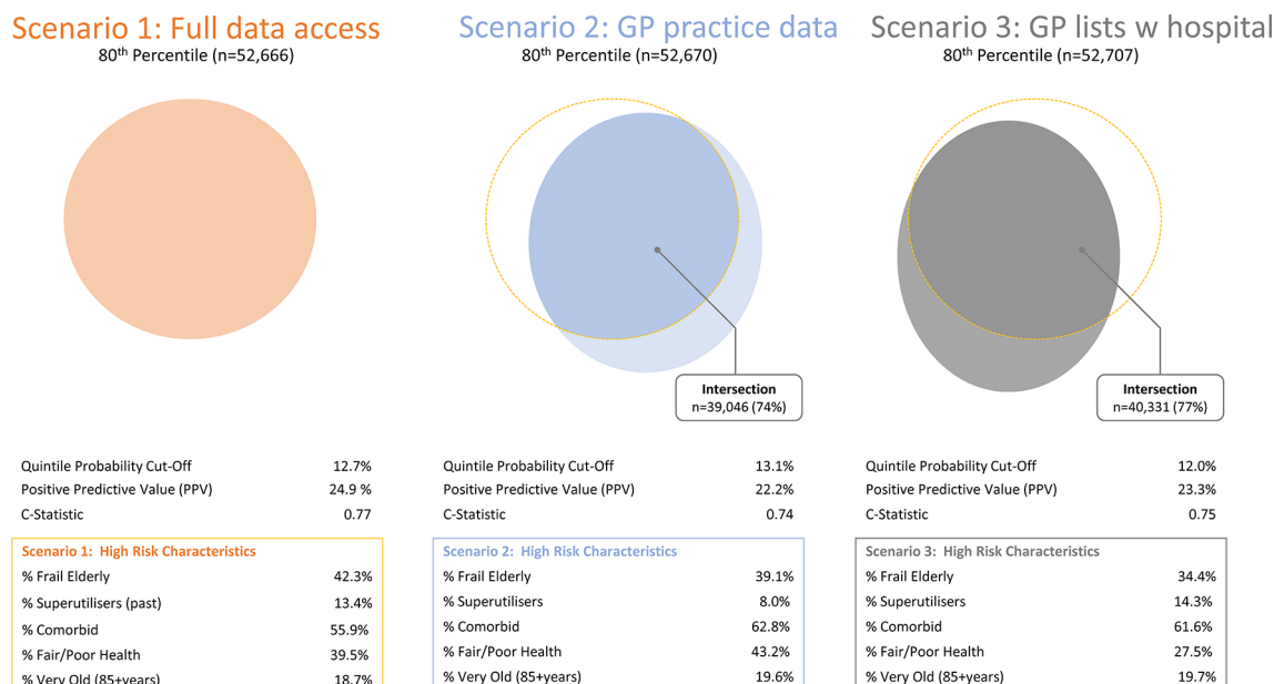
Figure 1 Comparison of high-risk quintiles from the full, GP and hospital scenarios. GP, general practice.
